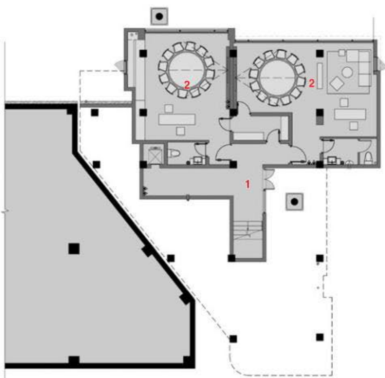
1st floor plan (Bldg. 5)
